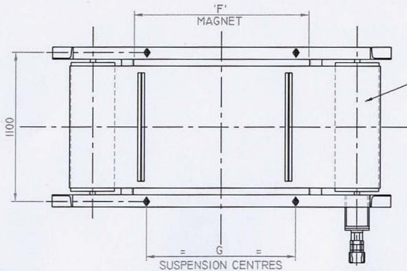
VIEW WITH HYDRAULIC DRIVE
